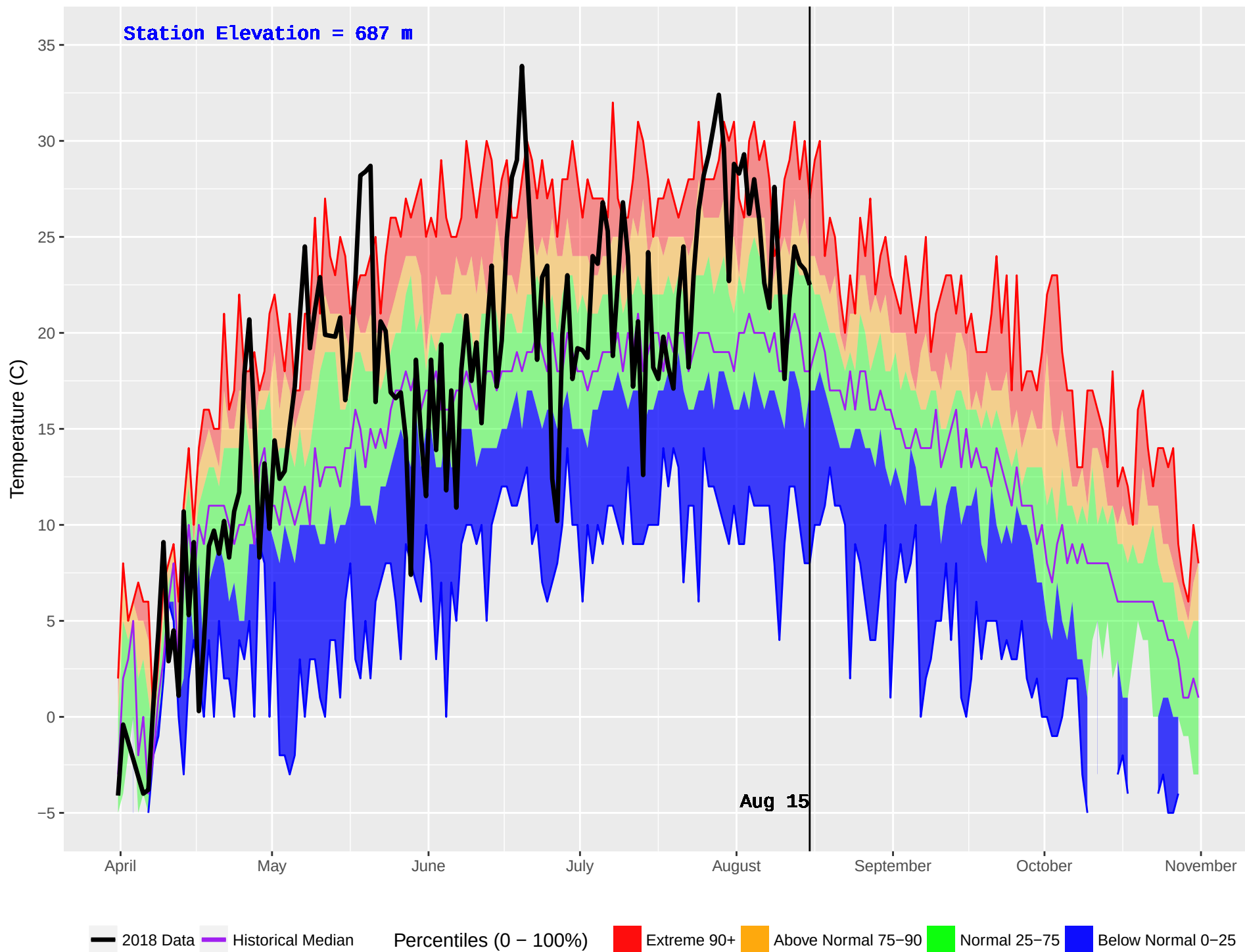
KETCHIKA (444) : Historical (1986–2016) and Current (2018) Daily Temperature
