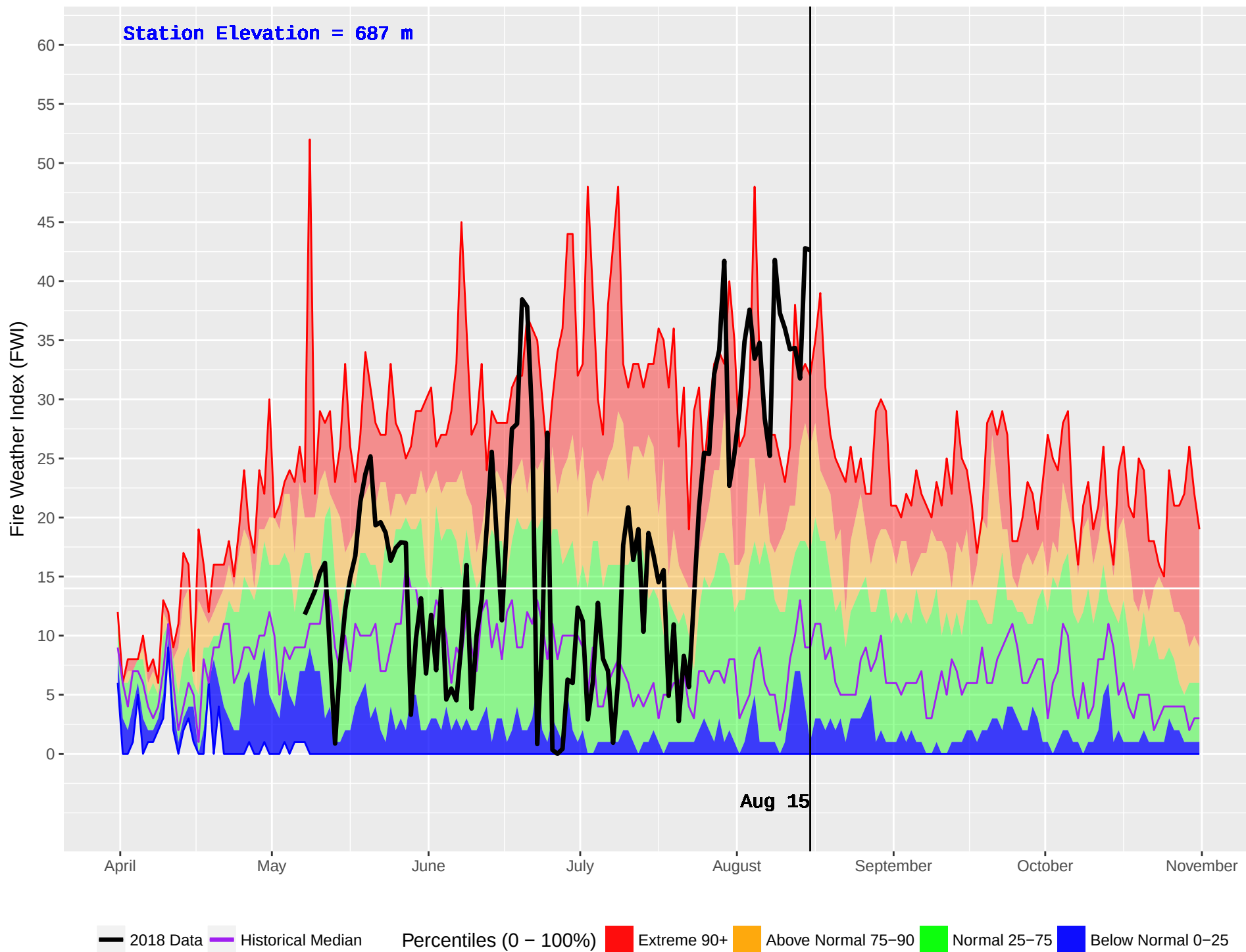
KETCHIKA (444) : Historical (1986–2016) and Current (2018) Daily Fire Weather Index (FWI)
