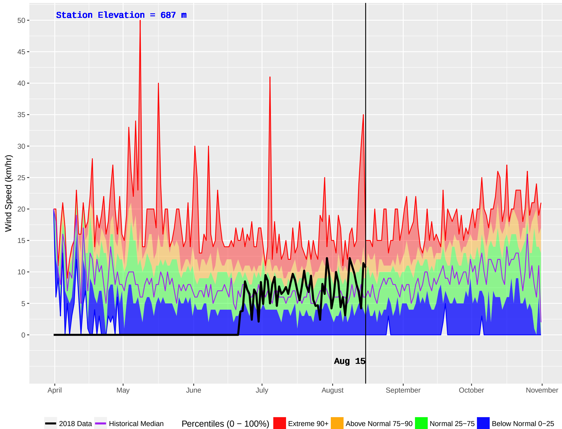
KETCHIKA (444) : Historical (1986–2016) and Current (2018) Daily Wind Speed
